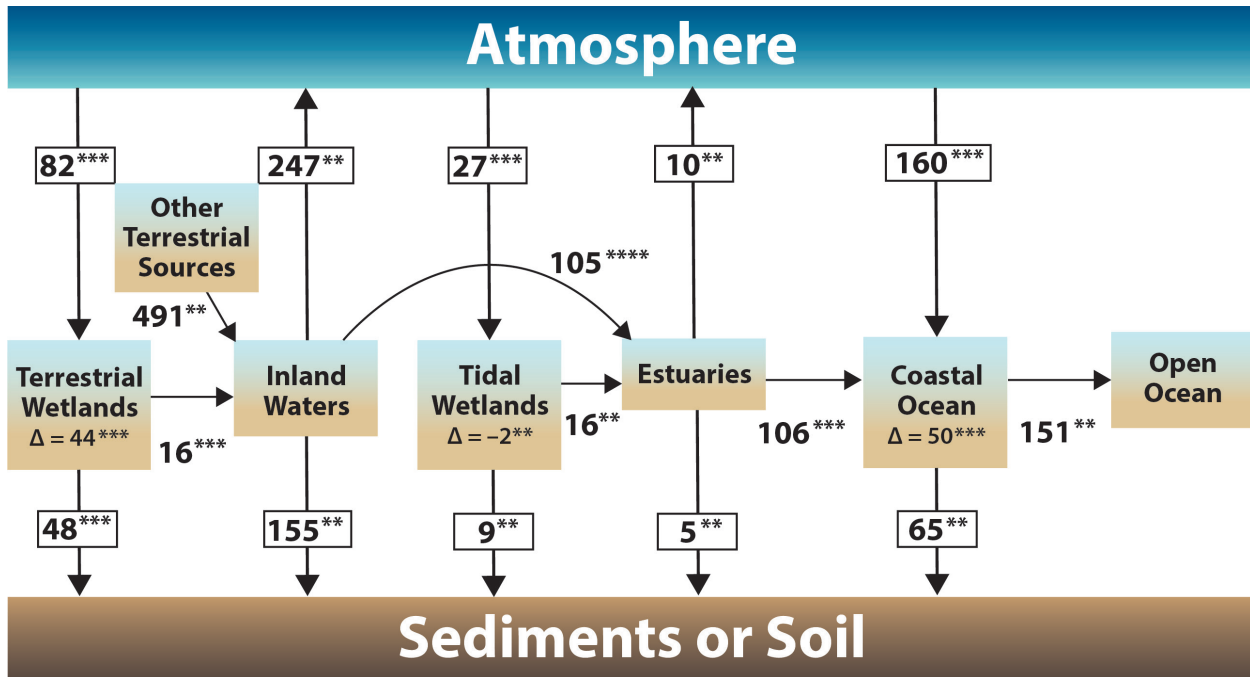
Figure ES.3. Total Carbon Budget of North American Aquatic Ecosystems. Flux estimates, in teragrams of carbon (Tg C) per year, are derived from Ch. 13: Terrestrial Wetlands, Ch. 14: Inland Waters, Ch. 15: Tidal Wetlands and Estuaries, and Ch. 16: Coastal Ocean and Continental Shelves. Carbon exchanges with the atmosphere are limited to carbon dioxide (CO 2 ) except for terrestrial wetlands, which include CO 2 and methane. Arrows leading from the atmosphere to different aquatic ecosystem compartments imply a loss of atmospheric carbon from the atmosphere to the ecosystem (a carbon sink). Arrows leading from the ecosystem to the atmosphere imply a loss of carbon from the ecosystem to the atmosphere (a carbon source). Horizontal arrows refer to transfer of carbon between ecosystems. Changes in some reservoir sizes are provided inside the boxes with deltas (Δ). Asterisks indicate that there is 95% confidence that the actual value is within 10% (****), 25% (***), 50% (**), 100% (*), or >100% (*) of the reported value.
