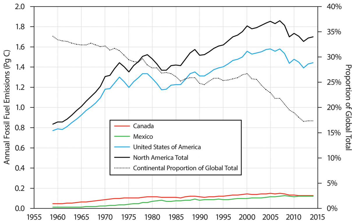
Figure ES.5. Annual North American Fossil Fuel Emissions from 1959 to 2014. Values are given in petagrams of carbon (Pg C) for each country and for the continent as a whole (solid lines, left vertical axis). The dotted line shows the North American proportion of total global emissions (right vertical axis). [From Figure 2.2 in Ch. 2: The North American Carbon Budget. Data source: Carbon Dioxide Information Analysis Center (Boden et al., 2017).]
