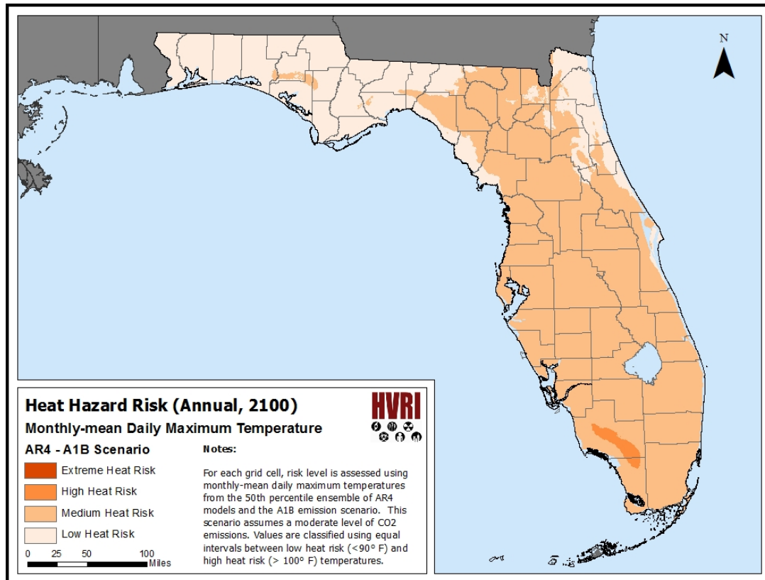
Figure 43: Monthly-mean daily maximum temperature for the A1B scenario in Florida, 2100.
