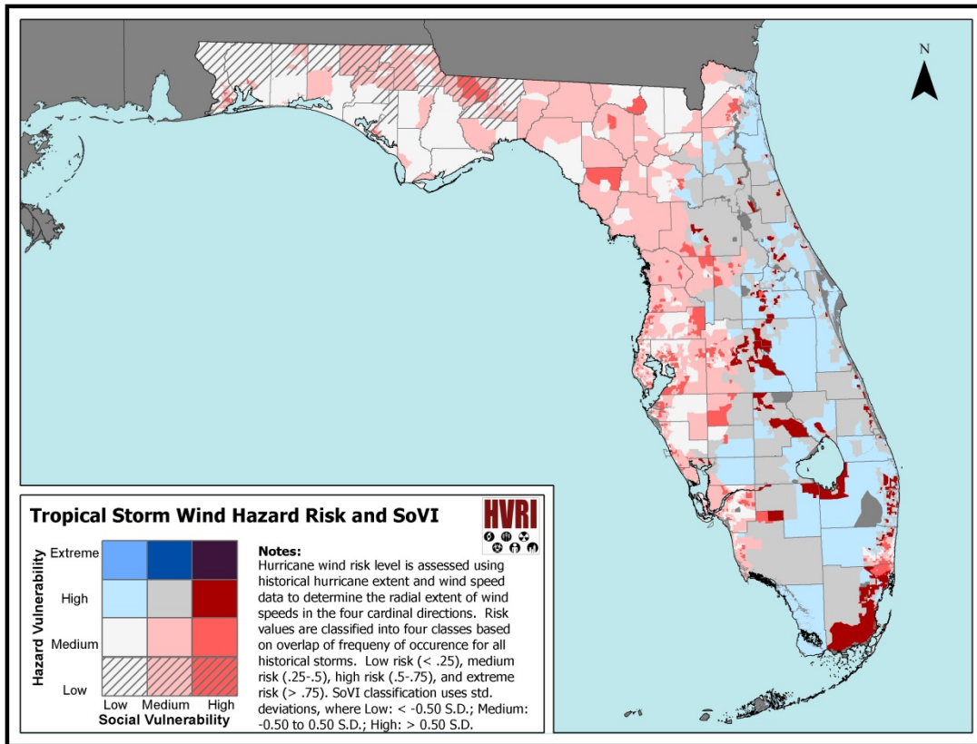
Figure 8: Bivariate representation of SoVI and tropical storm force wind hazard risk in Florida
