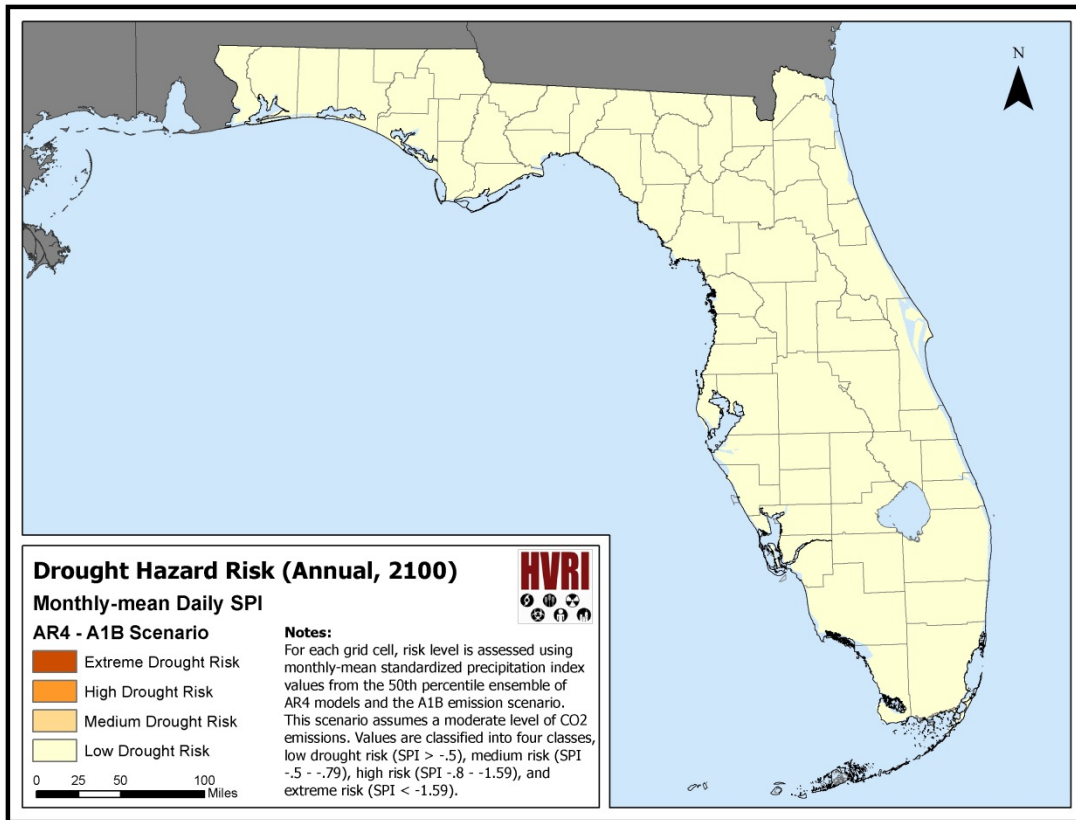
Figure 56: Monthly-mean daily SPI for A1B scenario in Florida, 2100.
