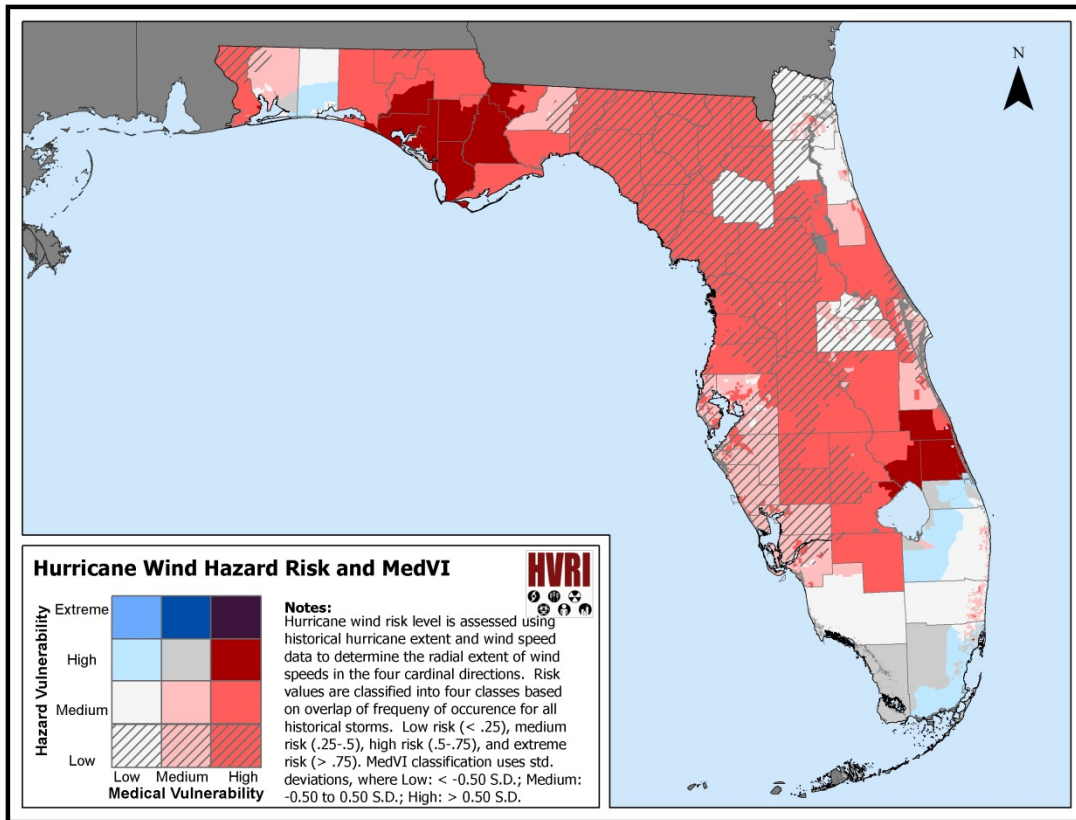
Figure 11: Bivariate representation of MedVI and hurricane force wind hazard risk in Florida.
