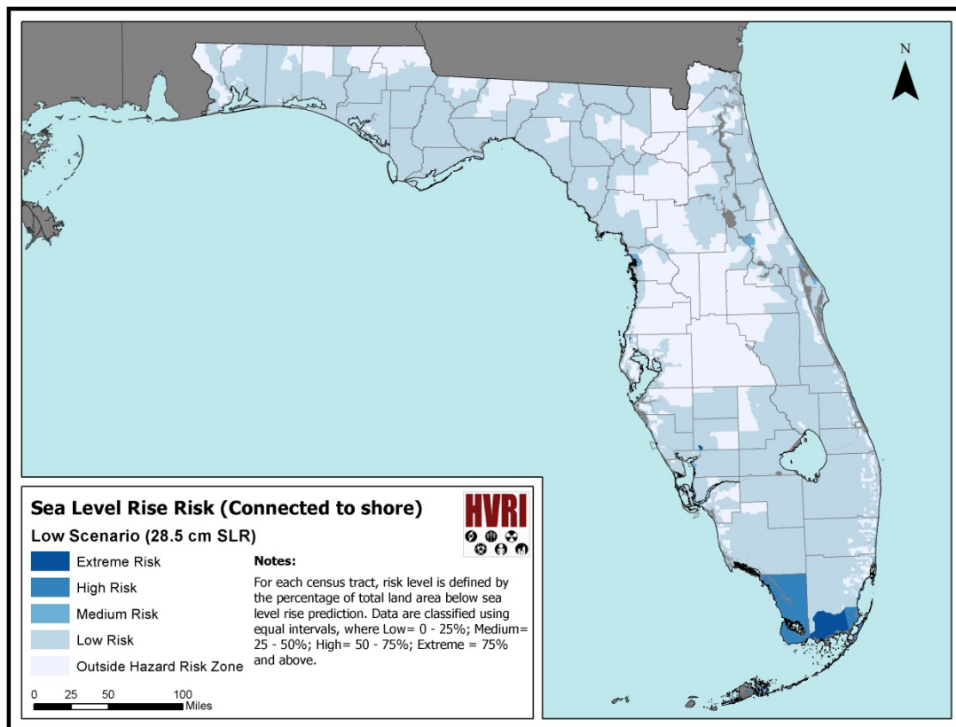
Figure 33: Sea level rise risk in Florida – low scenario (28.5 cm by 2100). Areas included are connected to the shore.
