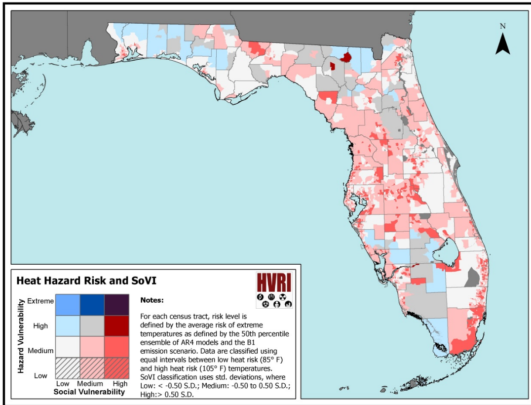
Figure 50: Bivariate representation of SoVI and heat hazard risk for B1 scenario in Florida.
