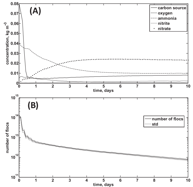
Fig. 8 – Average concentration of substrates (A) and number of flocs (B) in the heterogeneous reactor for the reference case runs (HRT = 0.3 d, SDT = 5.1 d).
