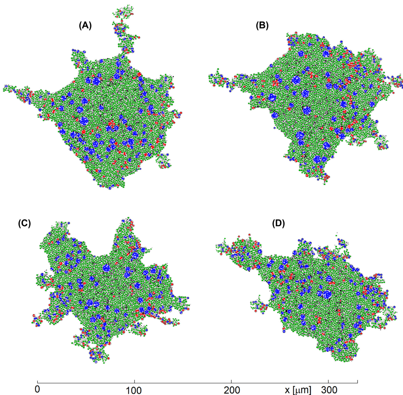
Fig. 11 – Various shapes of flocs obtained at Day 10 simulated time, for different solid dilution times (SDTs). (A) SDT 9.5 days; (B) SDT 11.32 days; (C) SDT 13.68 days; (D) SDT 16.88 days.
