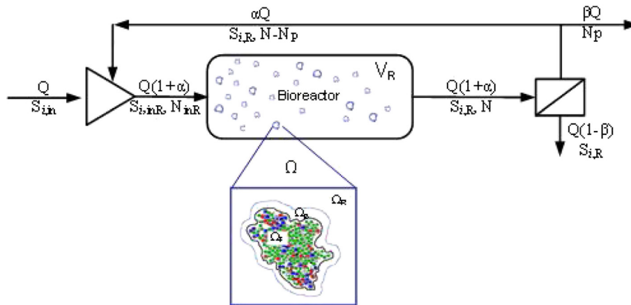
Fig. 1 – The scheme of the reactor–separator system considered in the mathematical model and the connection between scales.
