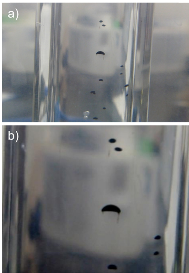
Figure 1. Video frame capture showing tip streaming from DH proxy crude oil mixed with COREXIT 9500 at 1:50 DOR during simulated buoyant rise: (a) original frame capture and (b) cropped and expanded. Buoyant droplets are stabilized for observation with a downward flow of synthetic seawater. Filaments of oil are shed from the edges of droplets (tip streaming) resulting in a rapid decrease in size. The width of the large crescent-shaped droplet is \sim 3 mm; it disappeared within 20–30 min, producing an ensemble of tiny droplets < \sim 100 \mu\text{m} . See Nagamine (2014) for more details. Contrast of images was adjusted for clarity.
