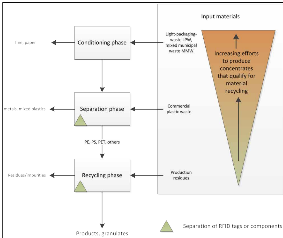
Figure 42. Steps in plastic recycling and applicable waste streams
