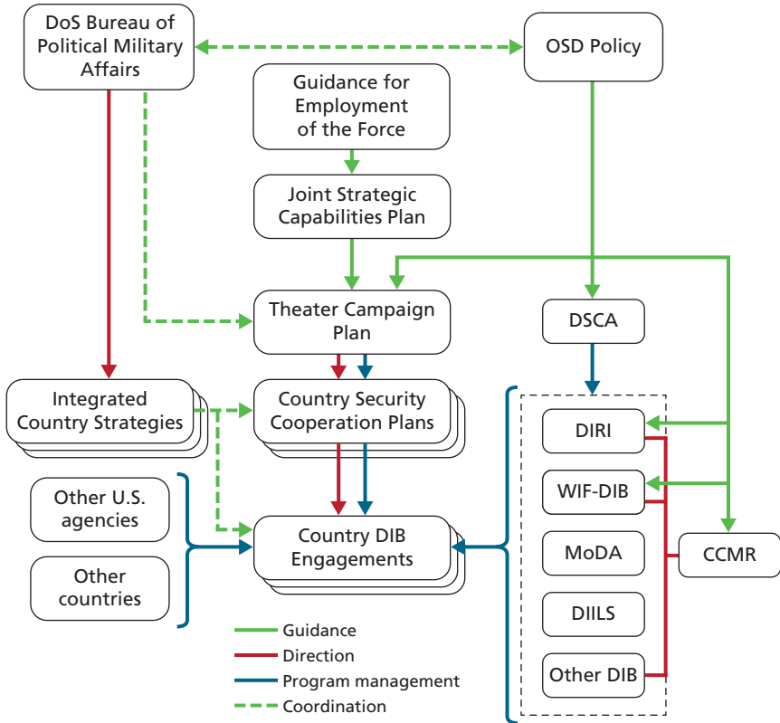
Figure 2.9 DIB Guidance
