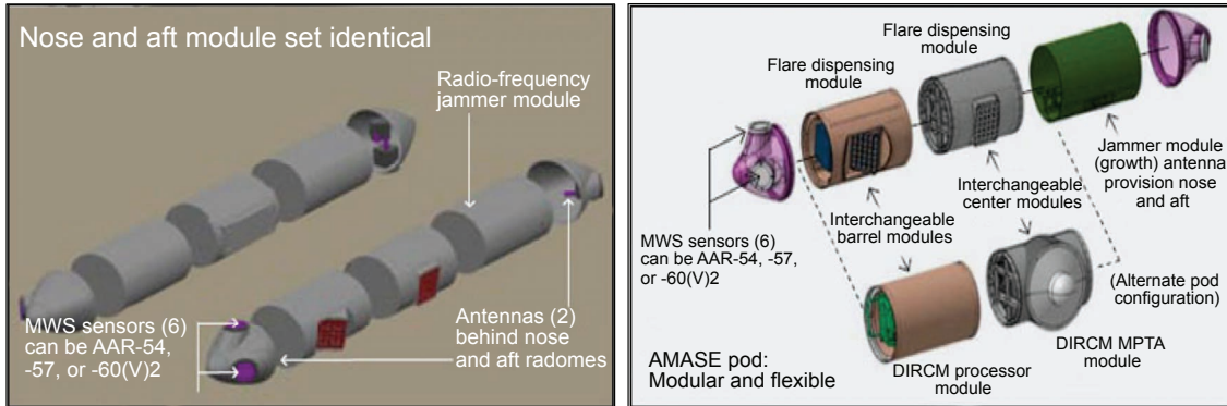
Danish Apache Modular Aircraft Self-Protection Equipment (AMASE)
