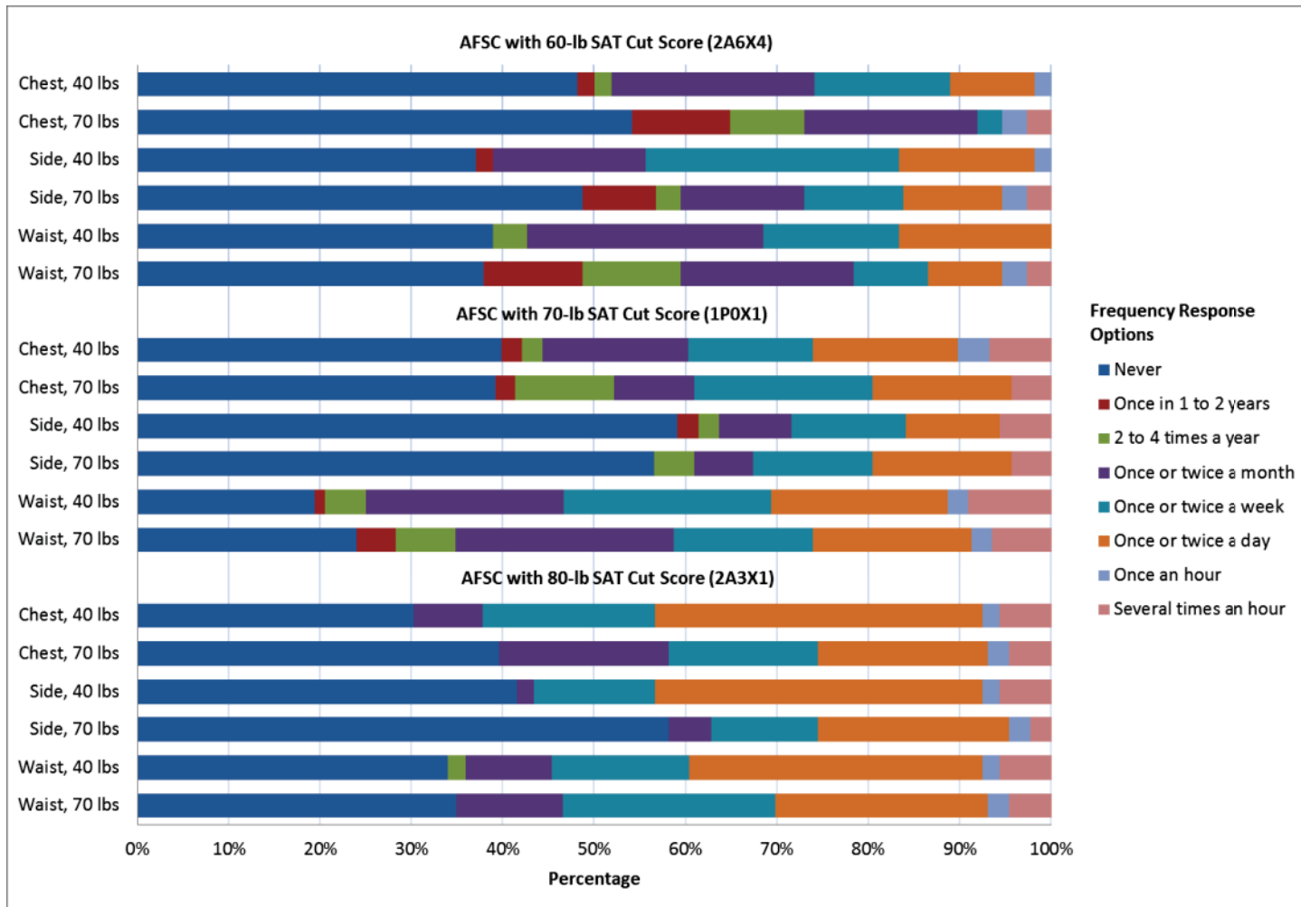
Figure 5.3 Frequency Ratings of Three Movement Types for Lift, for Three AFSS
