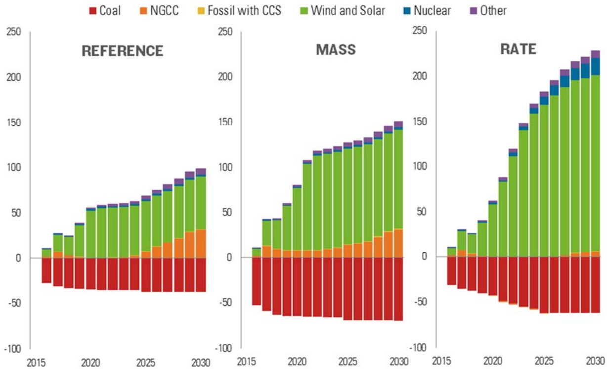
Figure 4. Generation change from 2015 (TWH)
