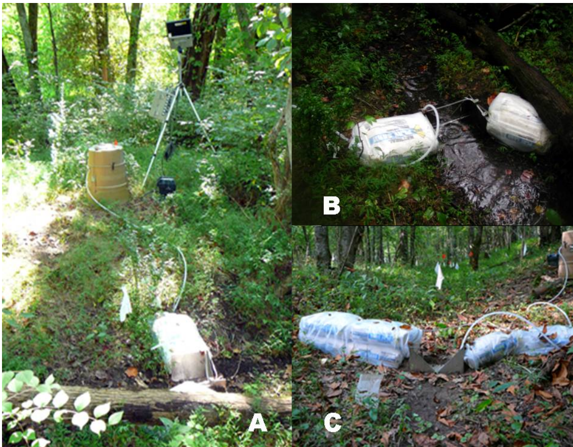
Fig. 8. Floodplain runoff sampling design for the wet-weather catchment study: (A) weir, ISCO sampler, and flow meter at the NOAA site; (B) close-up of weir at the NOAA site during a rain event; (C) view through weir at the Horizon Center site showing floodplain wet-weather catchment.
