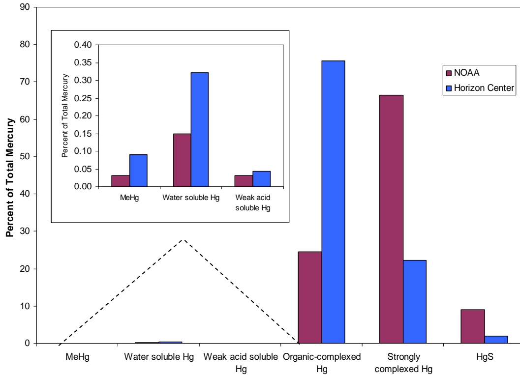
Fig. 18. Speciation of mercury in EFPC floodplain soils at the NOAA and Horizon Center floodplain study sites. Sequestered mercury (organic-complexed, strongly complexed, and HgS fractions in the sequential extraction speciation analysis) are to the right of the figure, while more accessible Hg species and methylmercury are shown in the inset to the left of the figure.
