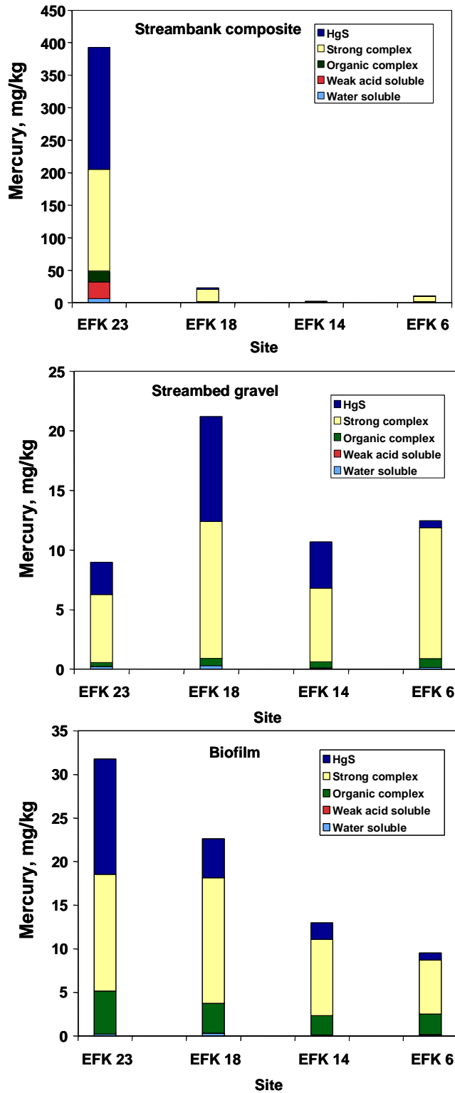
Fig. 13. Speciation of inorganic mercury in samples of streambank, gravel, and the surface biofilm of EFPC at sites along a downstream gradient. Numerical values for all fractions are presented in Table 5.
