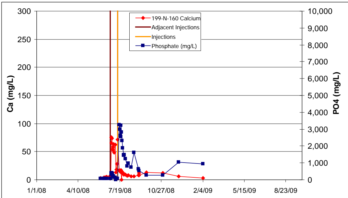
Figure B.19. Performance Plots for Well 199-N-160
