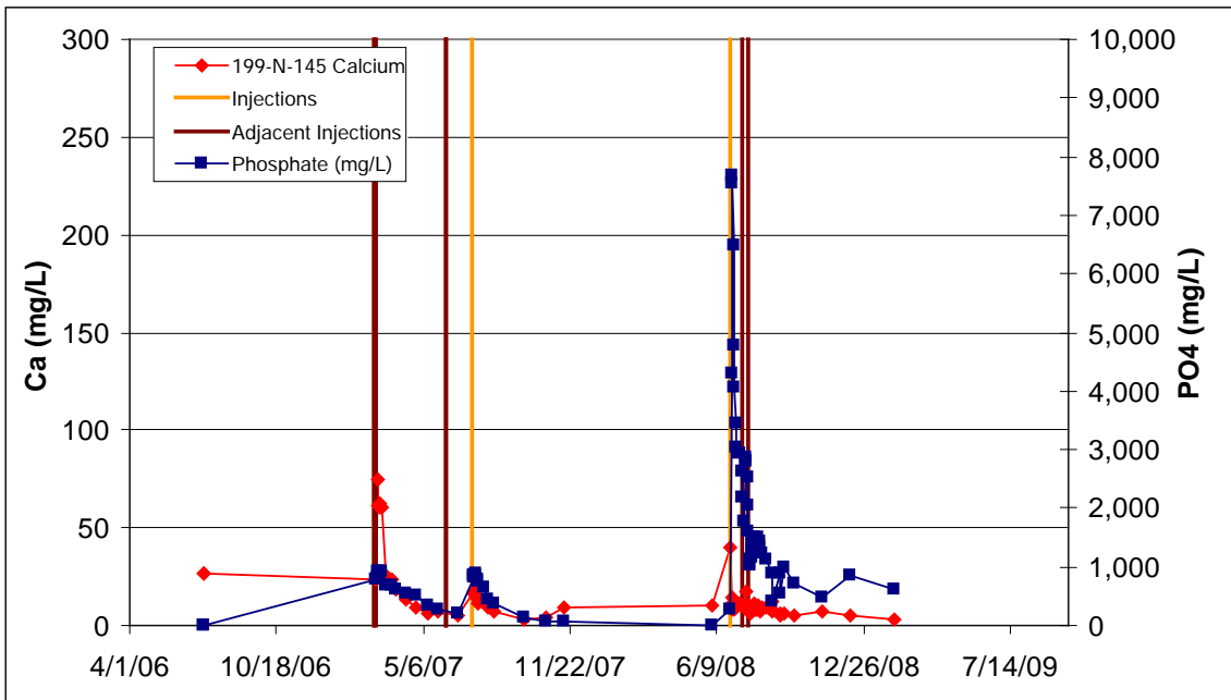
Figure B.18. Performance Plots for Well 199-N-145
