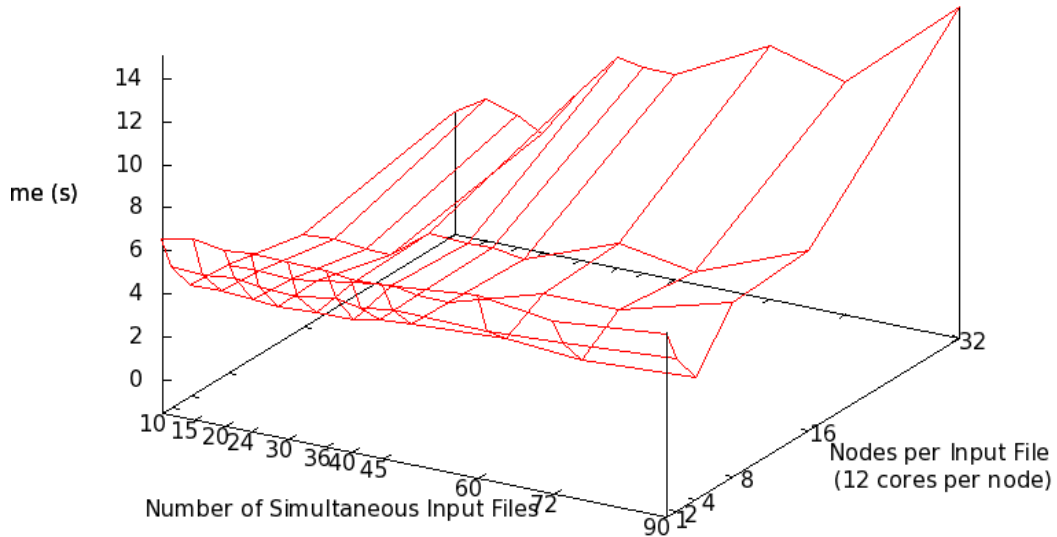
Figure 2: VTK reader time as a functional number of temporal regions and compute resources
