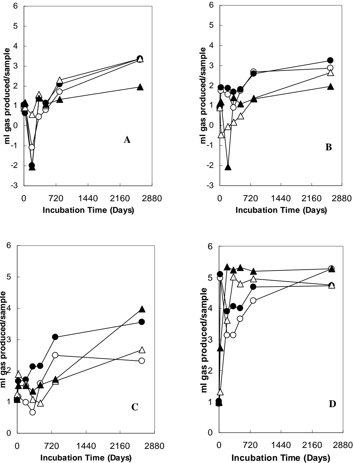
Figure 27. Total gas produced in samples containing polyvinylchloride: aerobic unamended (A); aerobic amended (B); anaerobic unamended (C); anaerobic amended (D). No polymer (○), unirradiated (●), low-dose (△), high-dose (▲).
