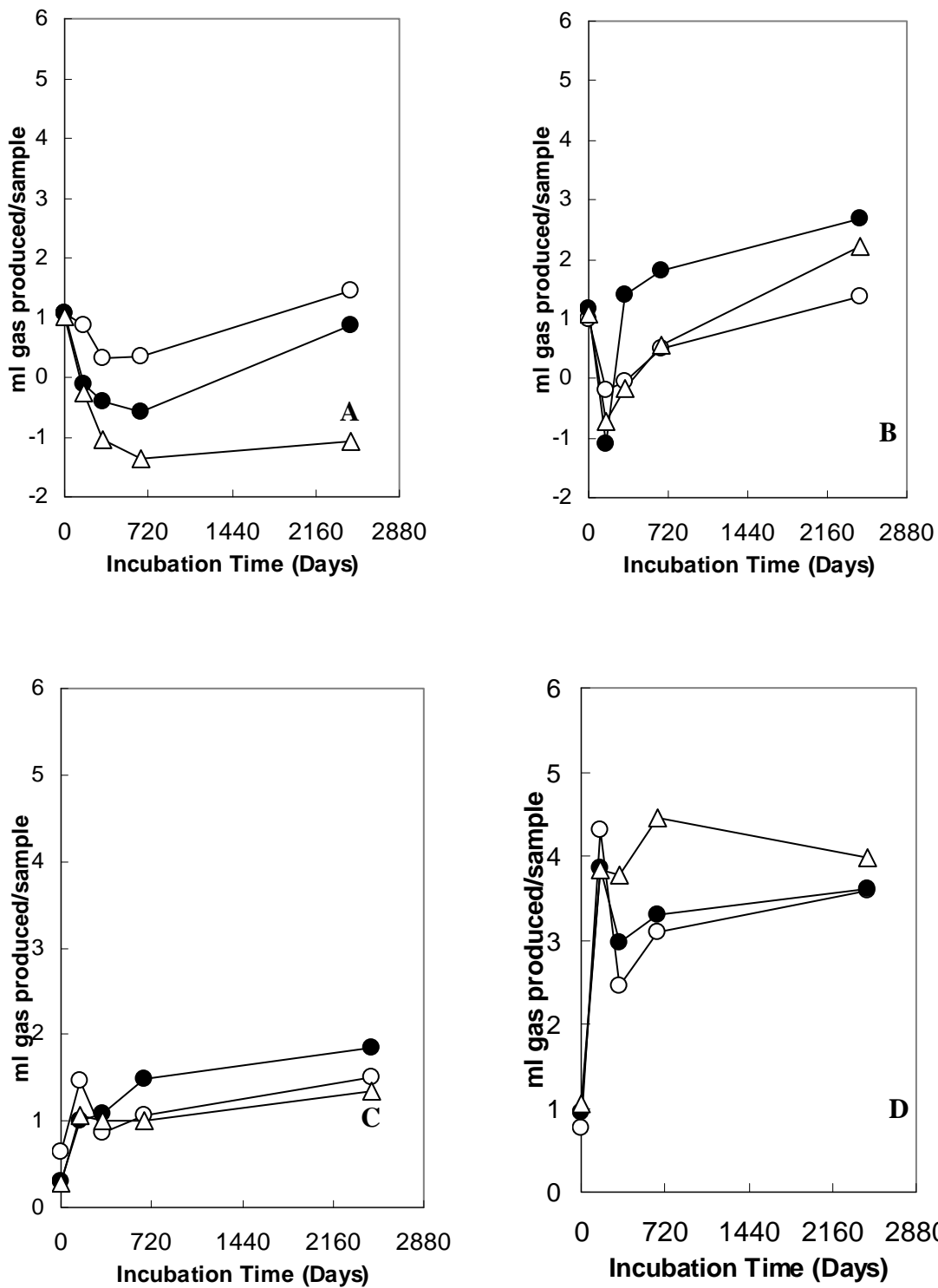
Figure 33. Total gas produced in samples containing leaded hypalon: aerobic unamended (A); aerobic amended (B); anaerobic unamended (C); anaerobic amended (D). No polymer (○), unirradiated (●), low-dose (△).
