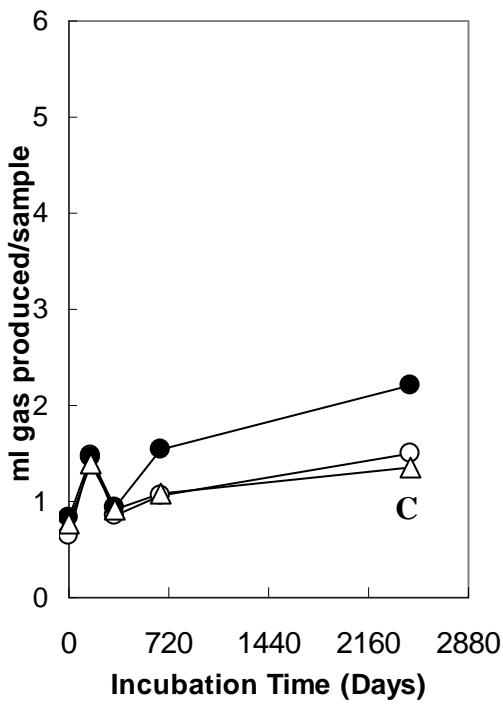
Figure 31. Total gas produced in samples containing unleaded hypalon: aerobic unamended (A); aerobic amended (B); anaerobic unamended (C); anaerobic amended (D). No polymer (O), unirradiated (●), low-dose (Δ).
