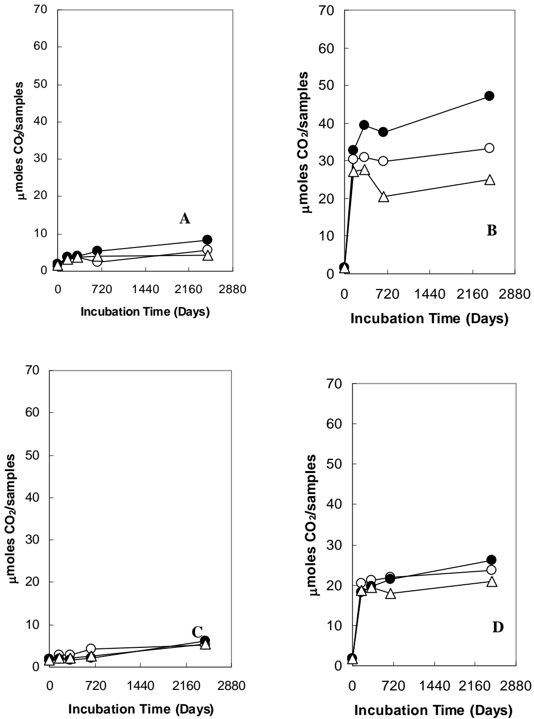
Figure 34. Carbon dioxide produced in samples containing leaded hypalon: aerobic unamended (A); aerobic amended (B); anaerobic unamended (C); anaerobic amended (D). No polymer (O), unirradiated (●), low-dose ( \Delta ).
