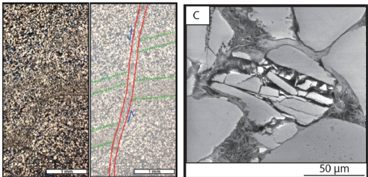
Figure 7. Left- micrograph mosaic for the Mount Simon Sandstone showing interpreted overlay of locations of compaction bands that are offset a small amount by a zone of cataclastic deformation bands. Right- grain-scale scanning electron microscopy image showing a shattered grain with surrounding authigenic clay cement.
