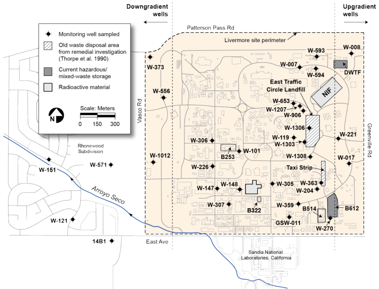
Figure 5-2. Routine surveillance groundwater monitoring wells at the Livermore Site, 2014.
