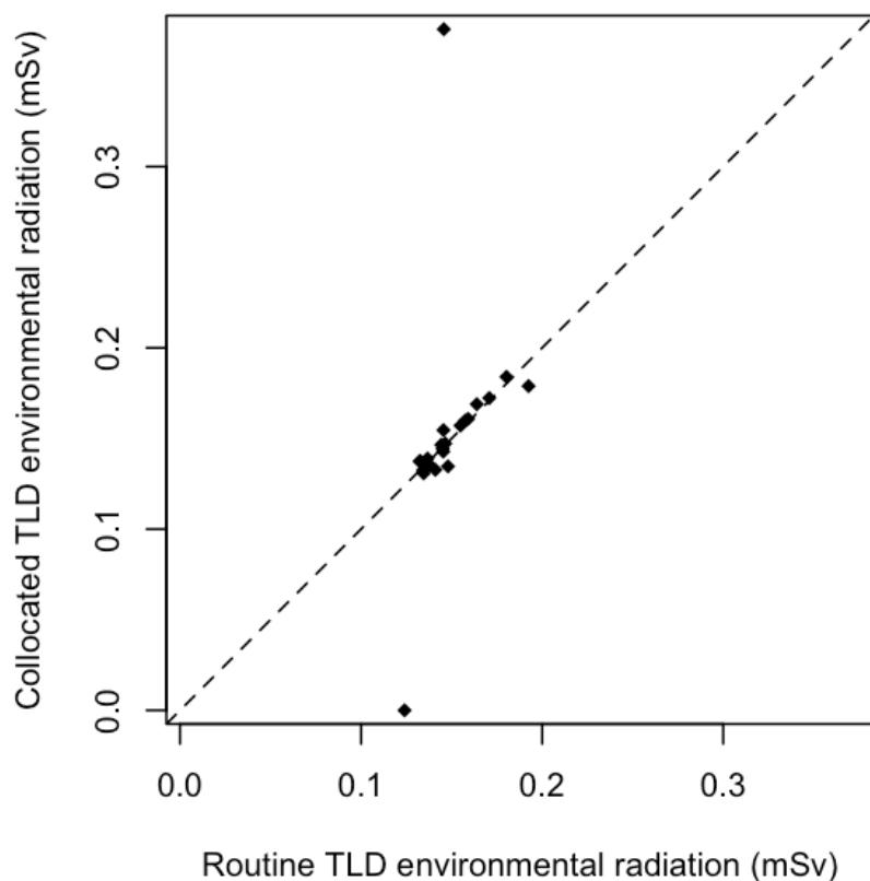
Figure 8-2. Example of data with two outliers using collocated direct radiation measurements.
