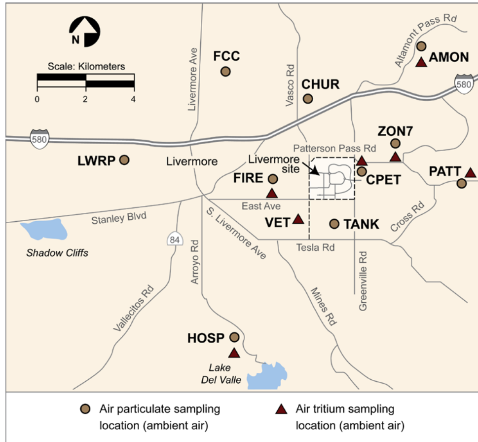
Figure 4-3. Air particulate and tritium monitoring locations in the Livermore Valley, 2014.
