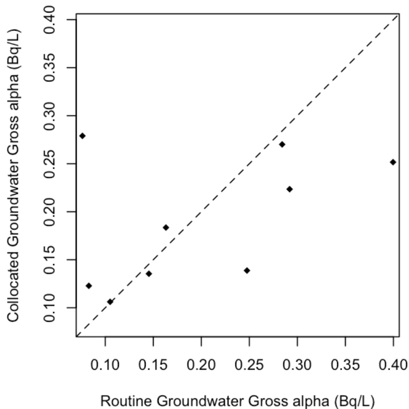
Figure 8-3. Example of high variability using collocated ground water gross alpha concentrations.
