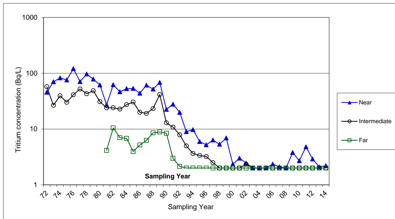
Figure 6-4. Median tritium concentrations in Livermore Site and Livermore Valley plant water samples, 1972 to 2014.
