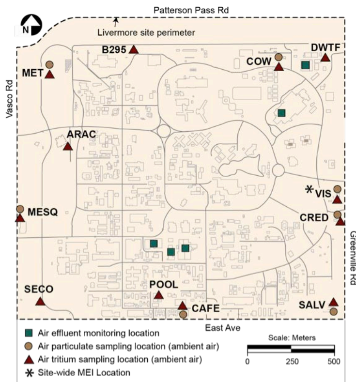
Figure 4-1. Air effluent and ambient air monitoring locations at the Livermore Site, 2014.
