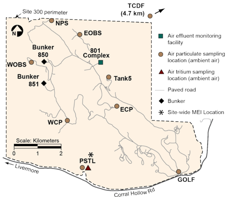
Figure 4-2. Air effluent and ambient air monitoring locations at Site 300, 2014.
