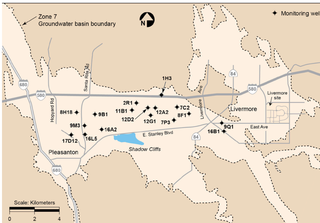
Figure 5-1. Off-site tritium monitoring wells in the Livermore Valley, 2014.
