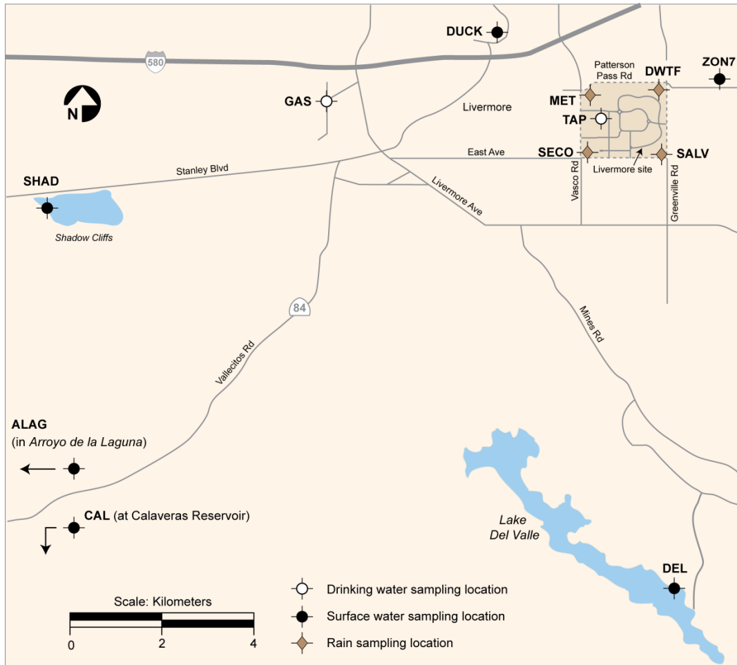
Figure 5-4. Livermore Site and Livermore Valley sampling locations for rain, surface water, and drinking water, 2014.
