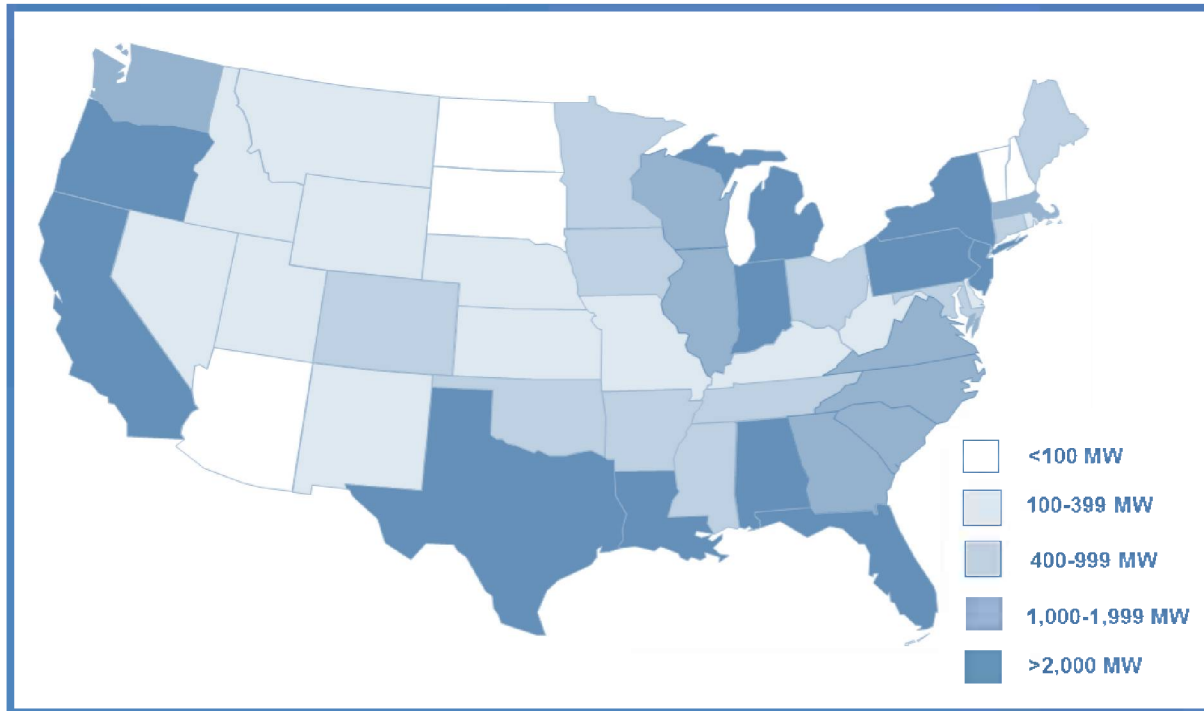
Figure 2. Existing CHP Installations (2014)
