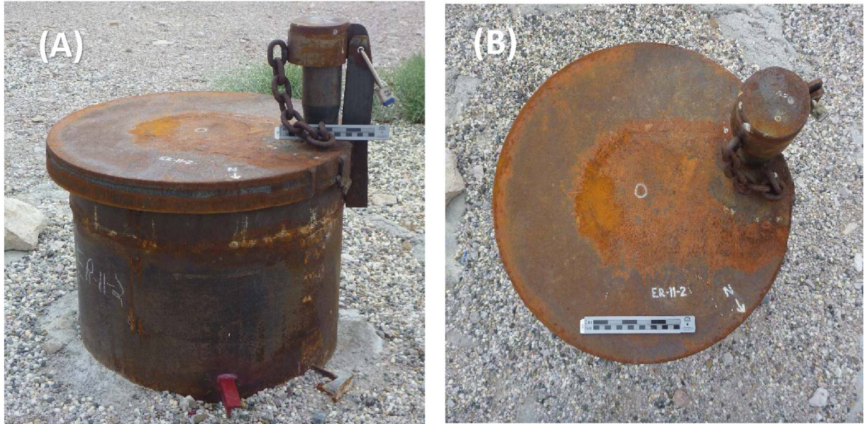
Figure 4. Photo of ER-11-2 wellhead configuration: (a) view to the south and (b) top-down view.
