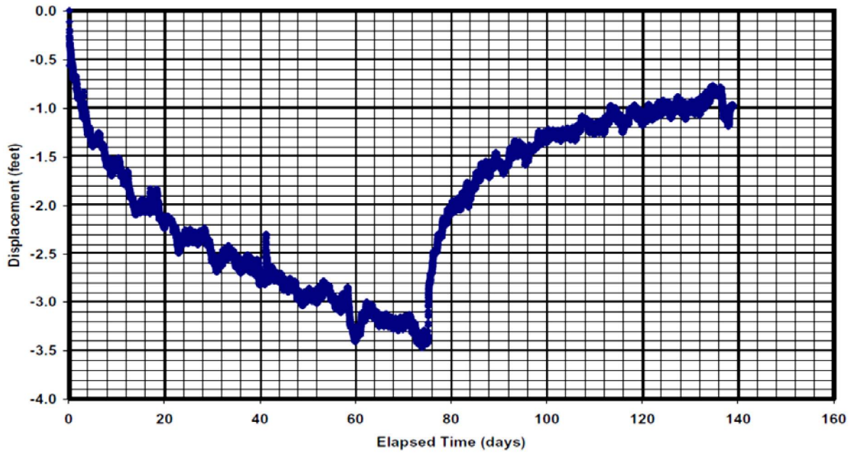
Figure 5-7 Drawdown Response Recorded for RNM-1 Corrected to True Vertical Depth
