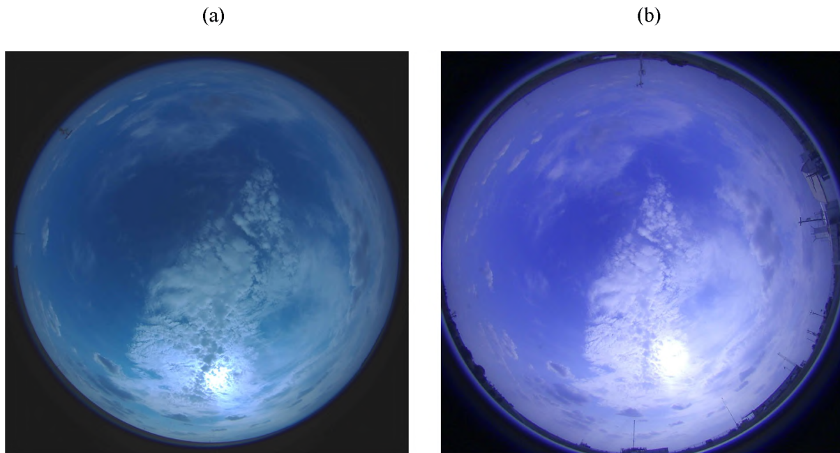
Figure 2. Examples of images collected by the BNL HD sky cameras. The images were collected by the two cameras separated by approximately 980 m at 21:04 UTC, September 29, 2015. Multi-layer clouds were evident from the images and the cloud base height is inversely proportional to the displacement of the cloud in the two images.
