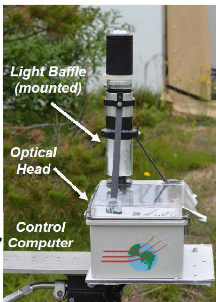
Figure 6. The TWST sensor hardware.
