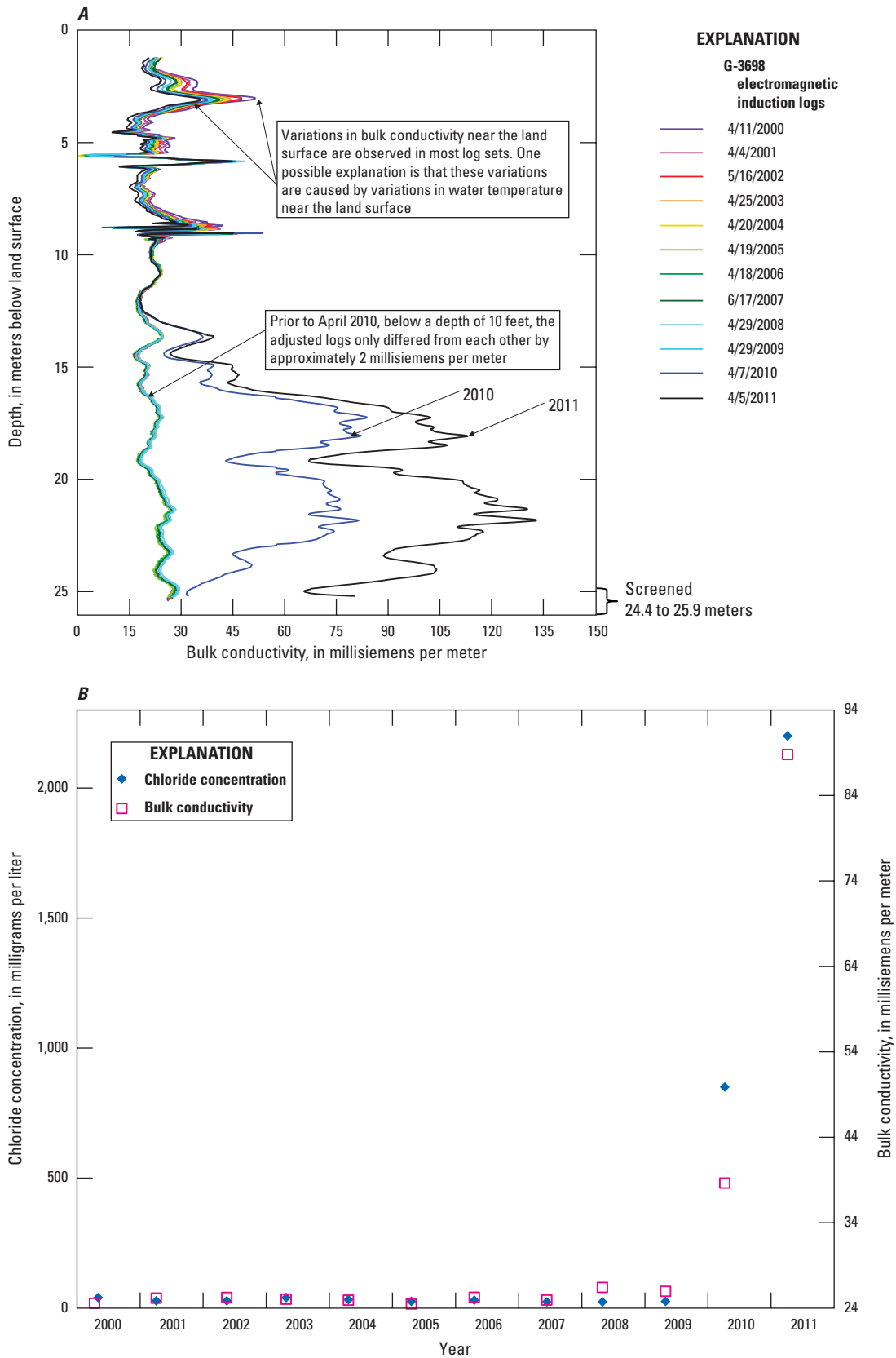
Figure 43. (A) Time-series electromagnetic induction log (TSEMIL) dataset; and (B) chloride concentrations in water samples from monitoring well G-3698 and bulk conductivity measured at a depth of 24.5 meters, Biscayne aquifer, Miami-Dade County, Florida.
