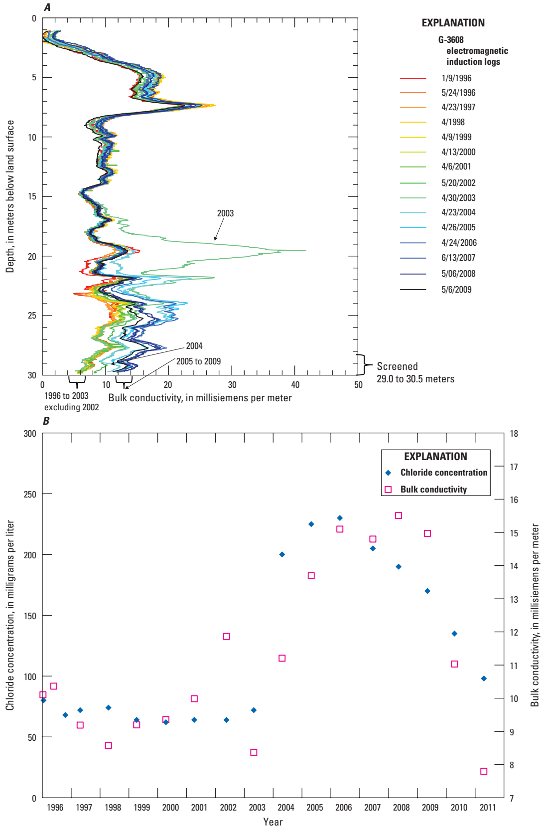
Figure 35. (A) Time-series electromagnetic induction log (TSEMIL) dataset; and (B) chloride concentrations in samples collected from well G-3608 and bulk conductivity measured at a depth of 28.9 meters, Biscayne aquifer, Miami-Dade County, Florida.
