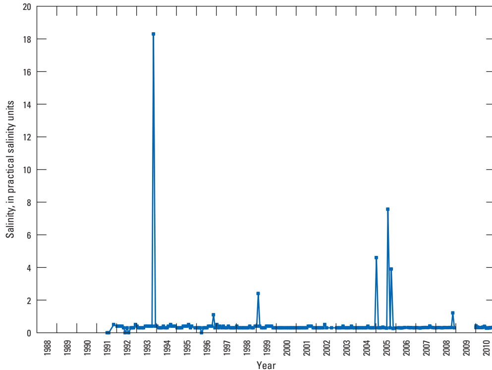
Figure 40. Salinity of the Princeton Canal at station PR03, 1991–2008 and 2010, Miami-Dade County, Florida.
