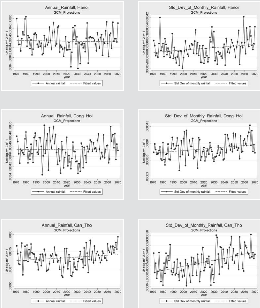
Figure A.3 Changes in Precipitation in Three Pilot Cities
