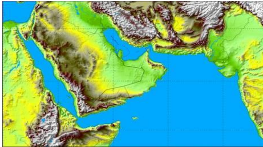
Figure 1: ORM_28km resolution domain
