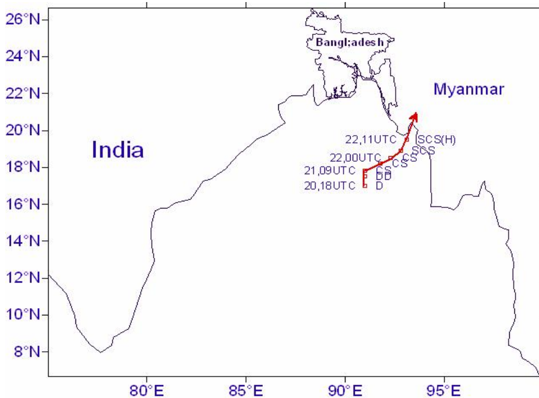
Figure 4: BMD observed track of severe cyclonic Storm 'GIRI' during 20-22 October 2010 of cyclone 'GIRI' October 2010
