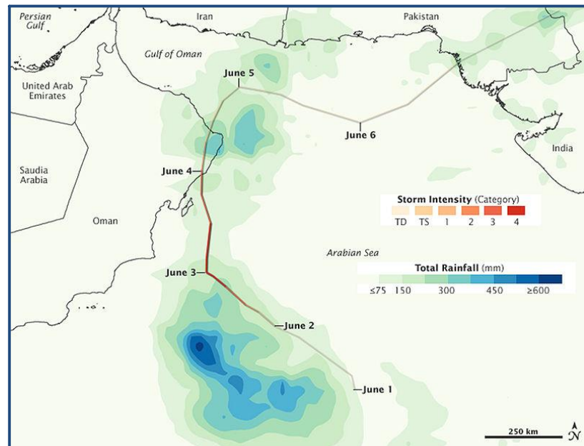
TRMM satellite rainfall estimate map (8 th June 2010) shows Cyclone Phet's heaviest rainfall (600 mm or 23.6 inches or more) occurred over open waters of the Arabian Sea (blue) Northeast Oman received as much as 450 mm (17.7 inches), while Pakistan received between 150-300mm / 5.9-11.8 inches. The colored line indicates storm track and intensity according to the Saffir-Simpson hurricane scale.
