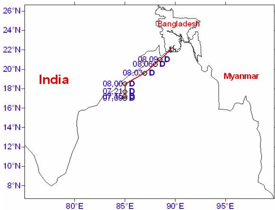
Fig. 2: BMD observed track of Depression during 07-08 October 2010.
