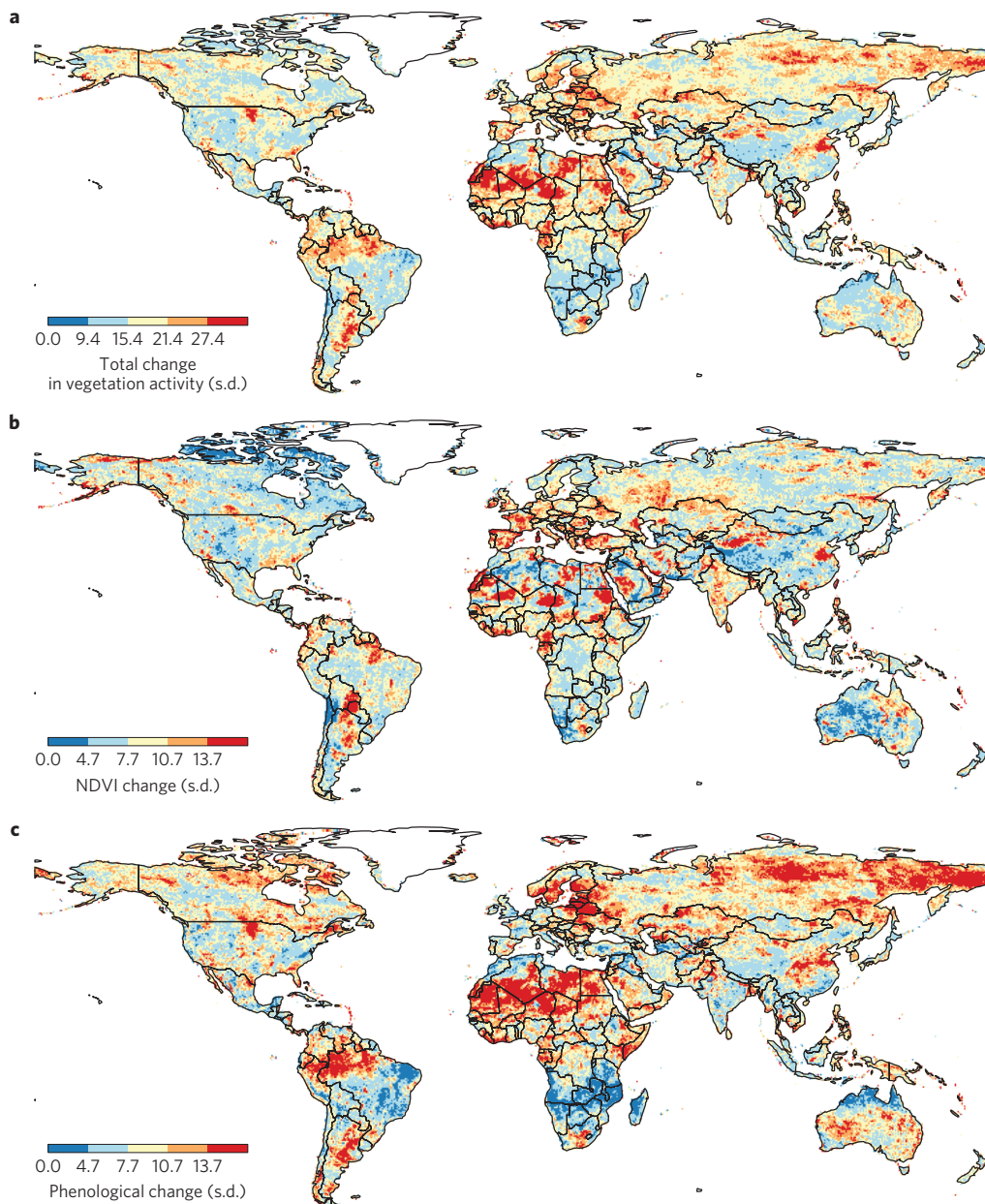
Figure 2 | Phenological change between 1981 and 2012. a, Total change in vegetation activity (the summed change of all 21 metrics). b, Change in the vigour of vegetation activity (the summed change of 10 metrics measured in NDVI). c, Change in the timing of the phenological cycle (the summed change of 11 metrics measured in days or day of year).
