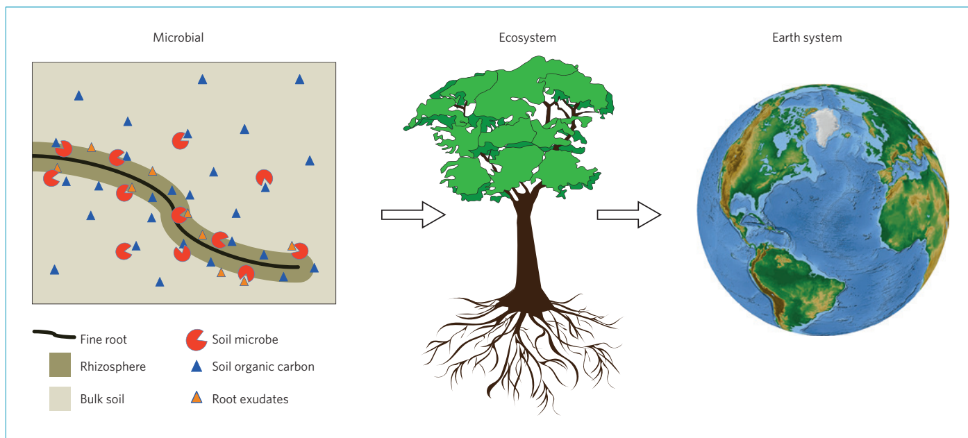
Figure 1 | Conceptual representation of the processes simulated by the CORPSE model. This model explicitly considers the microbial decomposition of soil organic matter in bulk and rhizosphere soils (near fine root surfaces). Additional inputs of easily decomposed carbon supplied by fine roots accelerate microbial activity and rates of biogeochemical cycling, processes that take place at microbial scales ( <10^{-3} m). At ecosystem scales ( \sim 1 to 10^6 m 2 ), increased concentrations of atmospheric CO 2 have been experimentally shown to effectively increase the volume of soils under rhizosphere influence. These insights have now been applied in a land surface model that runs at global scales (grid cell area >10^{10} m 2 ).
