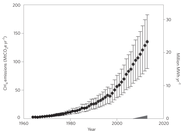
Figure 1 | Methane emissions from palm oil wastewater are an untapped bioenergy resource. Global scale \text{CH}_4 emissions and electricity potential were calculated by applying \text{CH}_4 emission and energy scaling factors to palm oil production statistics (Supplementary Tables 1–4 and Excel database). Error bars reflect the uncertainty in \text{CH}_4 emissions at 95% confidence intervals based on potential variation in wastewater treatment conditions at mills throughout the tropics (Supplementary Table 4). We estimate that 5% of mills capture POME bioenergy pantropically (shaded portion).
