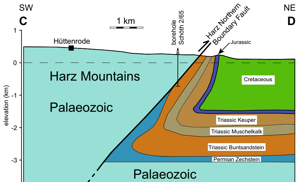
Fig. 4 Simplified cross section of the northern boundary of the Harz Mountains near Hüttenrode (see Figs. 2 and 3 for location). Diagram modified after Franzke et al. (2004)
