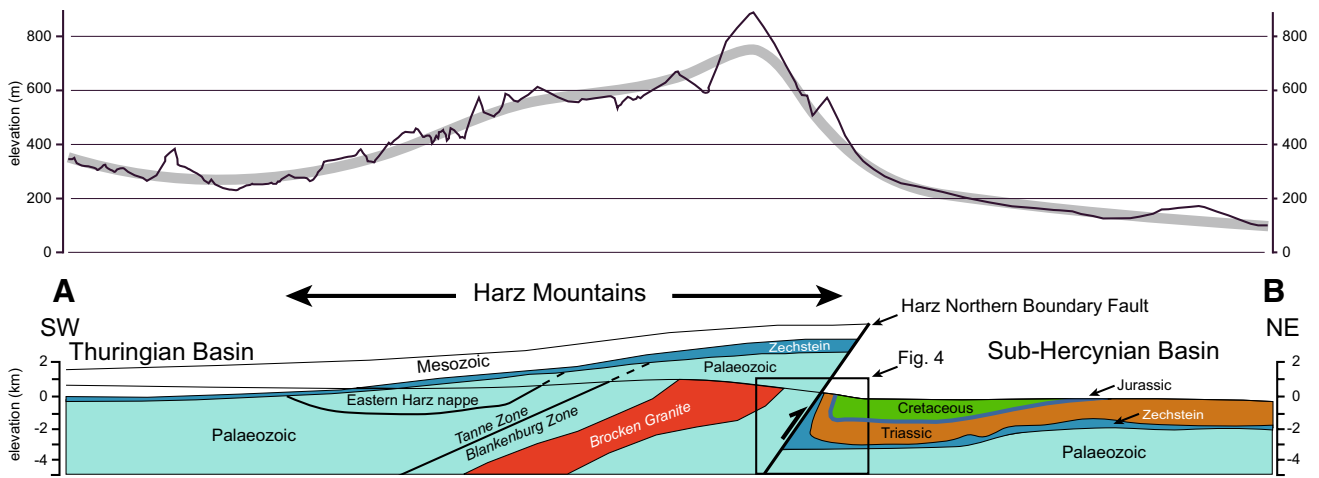
Fig. 3 Above topographic elevation taken from Google Earth, grey line—moving average (window 500 m). Below simplified cross section of the Harz Mountains, after Kley et al. (2008). Location of Fig. 4 is projected 15 km east (see Fig. 2 for location)
