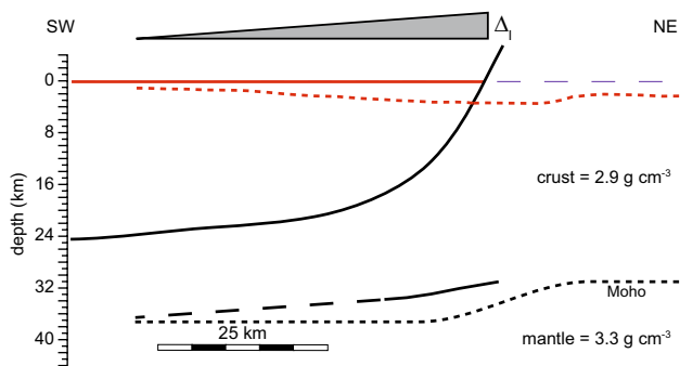
Fig. 8 Airy–Heiskanen isostatic equilibrium adjustment of the restored hanging wall in Fig. 7. Densities of the crust and mantle used in this work are shown. The triangle represents the amount of isostatic adjustment, where \Delta_I is calculated using Eq. 2. Dashed and solid lines represent Moho ( black ) and the surface topography ( red ) in the model, before and after isostatic equilibrium, respectively
