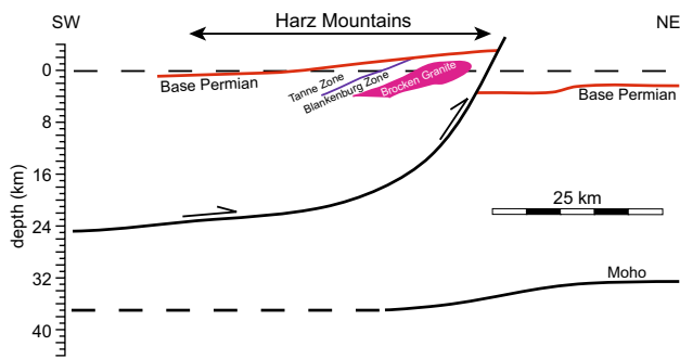
Fig. 6 Present-day cross section of the Harz Mountains with detachment of the main thrust at ca. 25 km depth, as predicted by 30° inclined-shear fault modelling
