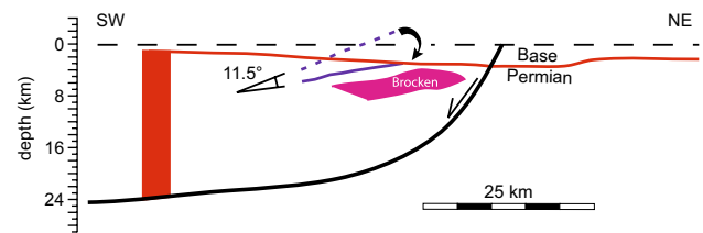
Fig. 7 Restoration of the Harz Mountains model to the Base Permian horizon using inclined shear. The dashed line represents the boundary between the Tanne and Blankenburg zones before restoration in Fig. 6; the clockwise rotation angle of 11.5° is caused by restoration
