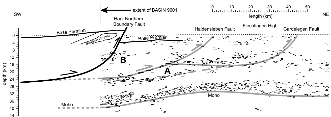
Fig. 9 Harz model presented in this paper together with the line drawing of the DEKORP BASIN 9601 seismic section. The Harz structure fits well with the detachment depths of the Gardelegen and
