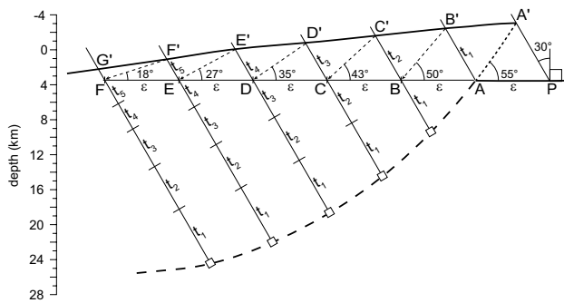
Fig. 10 Inclined-shear method to predict the shape of the fault using the hanging-wall geometry, the footwall/hanging-wall cutoffs, and a specific shear angle, here 30^\circ . Solid lines represent trace of Base Permian horizon, fine dashed thick line —known trace of the fault. Finely-dashed lines represent material vectors within the hanging wall. The angle of the material vector from the horizontal is given
